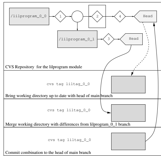
Figure 8: Update, merge and commit.
