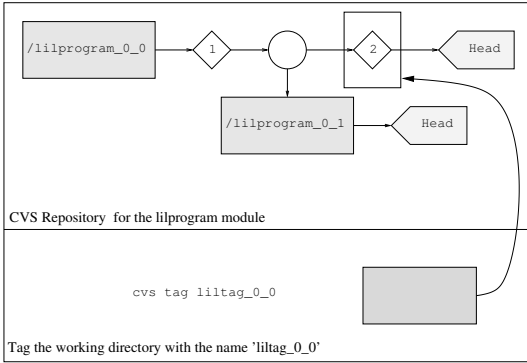
Figure 7: Tag the working directory.
