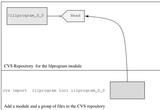
Figure 1: Import (legend is available page 9)
