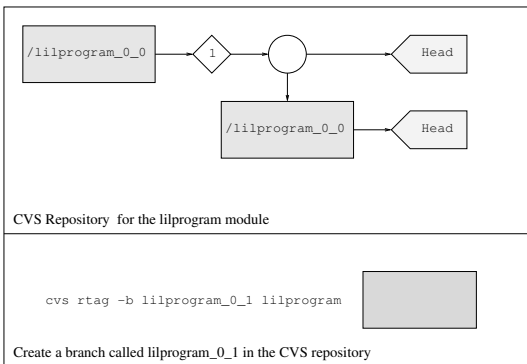
Figure 5: Create a new development branch.
