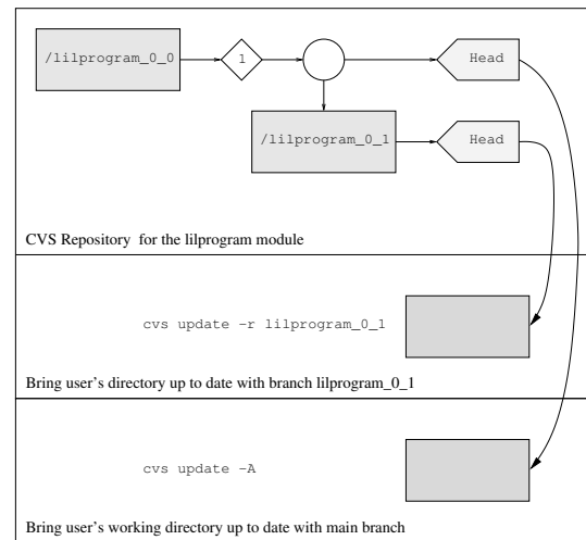
Figure 6: Update user's directory in function of the chosen development branch.
