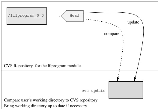
Figure 3: Compare and Update
